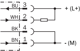
NPN dark-switching
