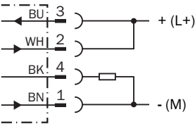
PNP dark-switching
