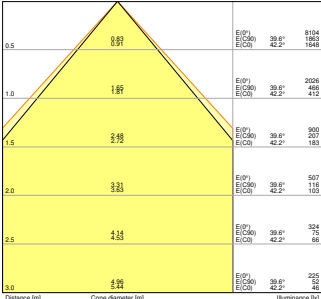
PL CMFT 600 P 30W 865 U19 PS
