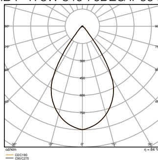
HB P 173W 840 70DEG IP66 PS - REFLECTOR
