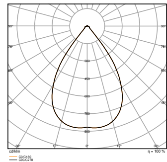
HB P 200W 840 70DEG IP66 PS
