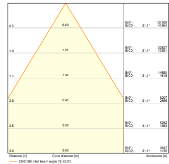
HB P 200W 840 70DEG IP66 PS - REFRACTOR
